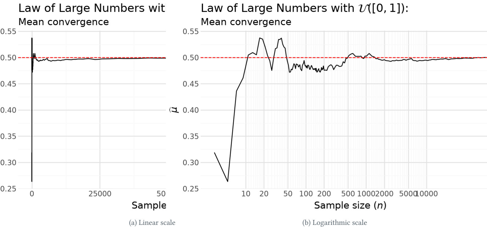
Figure 2: Convergence of the mean to the theoretical expectation (Question 3, Tip 1)
