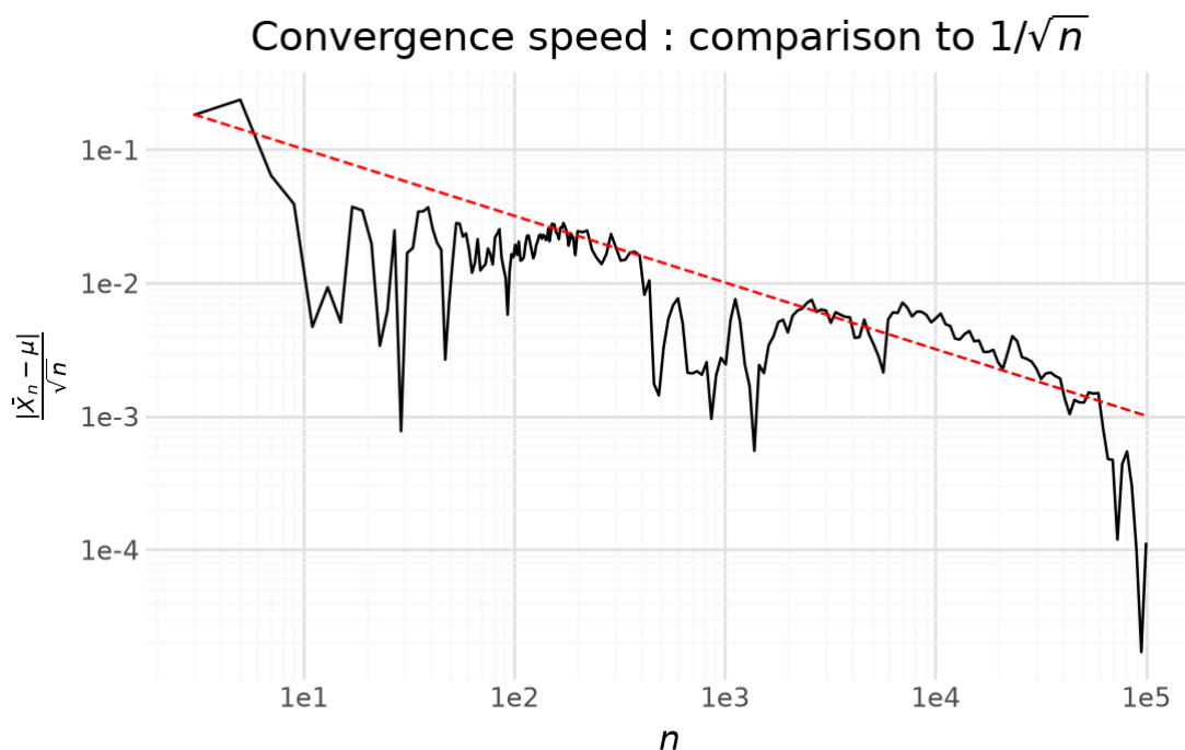
Figure 4: Plot of the estimation error and its relationship with the number of observations
