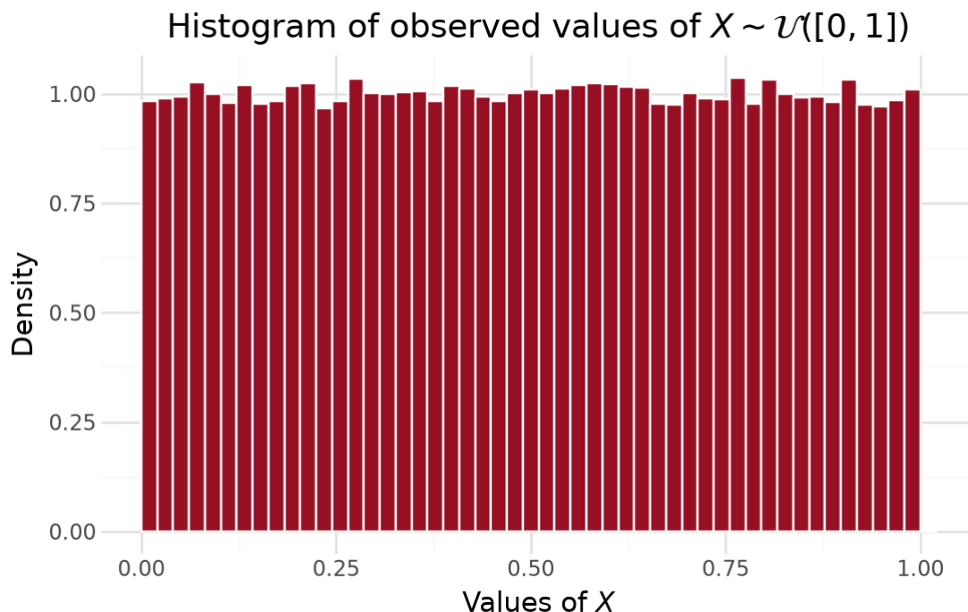
Figure 1: Empirical distribution of our random draw from the uniform law (Question 2, Tip 1)
