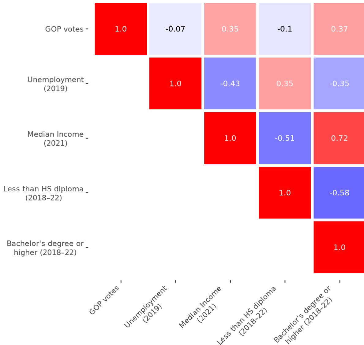
Figure 3: Correlation matrix with plotnine
