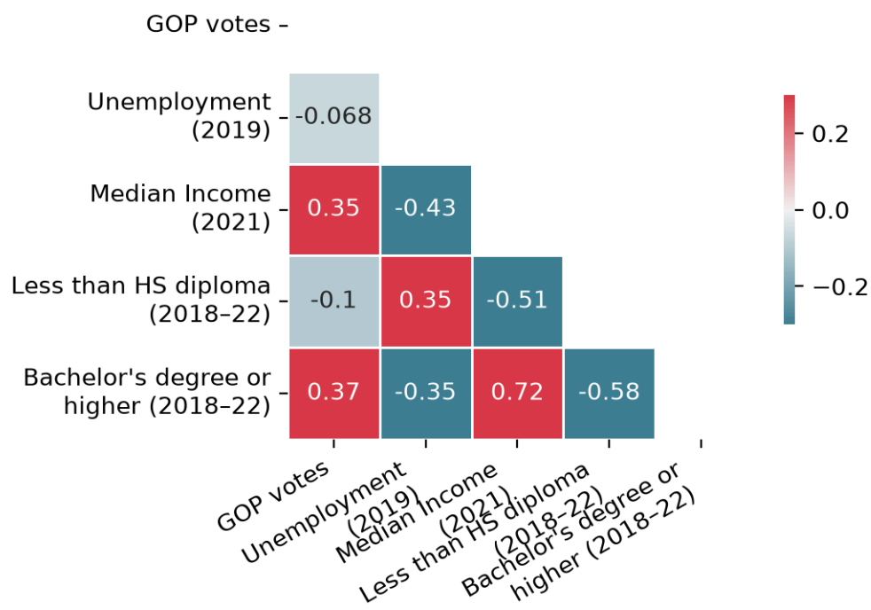
Figure 2: Correlation matrix with seaborn
