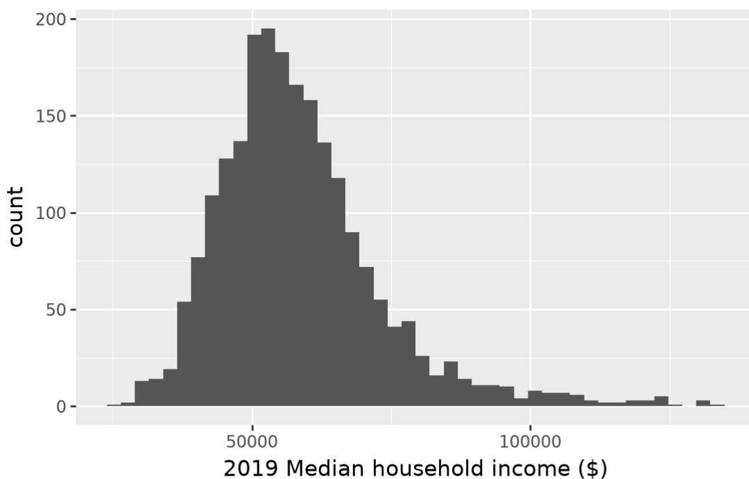
Figure 5: Question 2, before normalization
