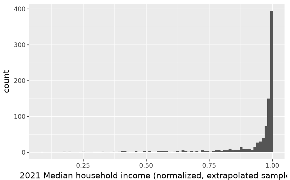
Figure 7: Question 2, transformed variable, using the trained parameters
