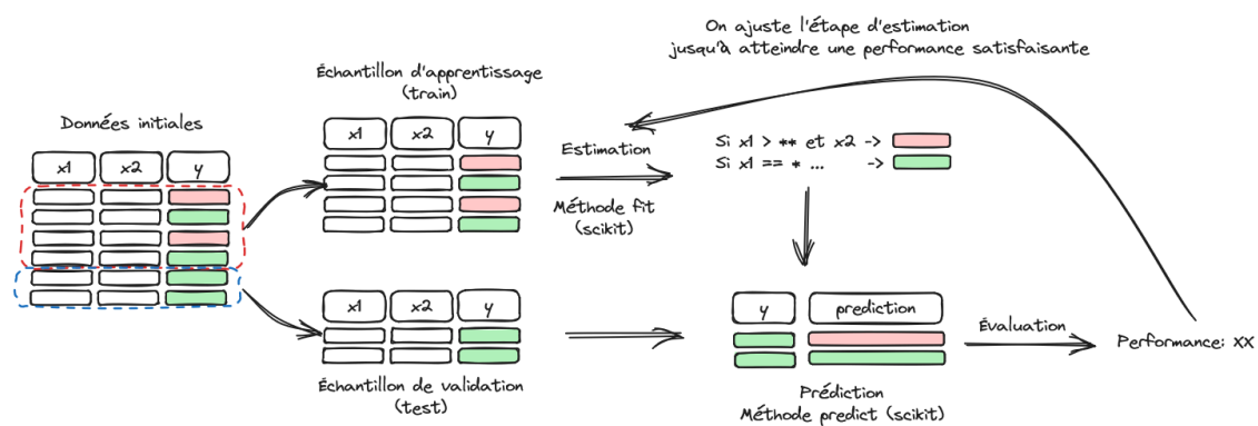
Figure 1: Illustration of machine learning methodology
