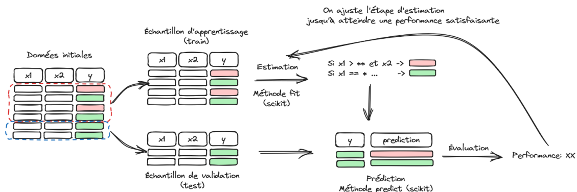
Figure 1: Machine learning methodology illustrated
