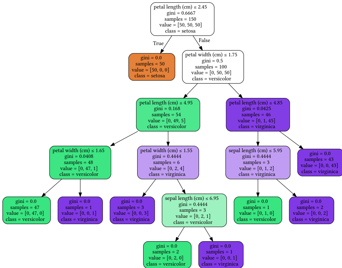
Figure 1: Example of a decision tree on the classic iris dataset. Source: scikit-learn documentation
