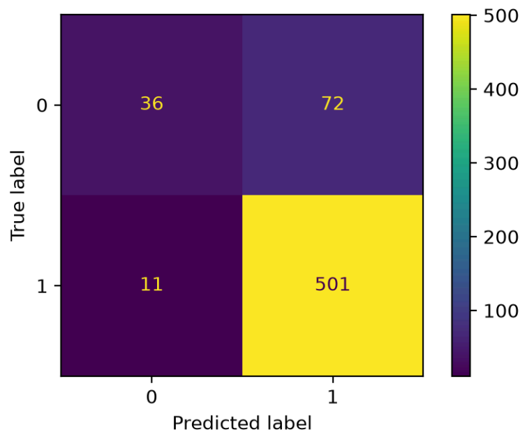
Figure 5: Confusion matrix for the best fitting model
