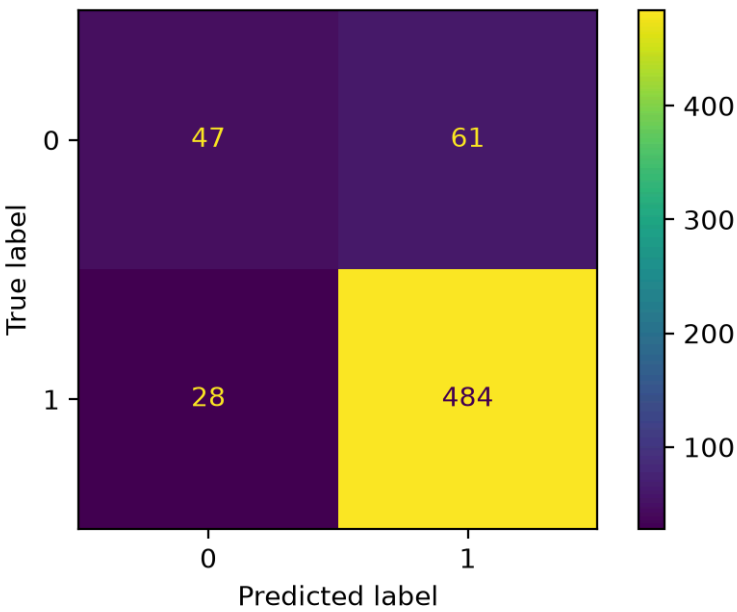
Figure 4: Confusion matrix from max_depth=4 decision tree (question 7)
