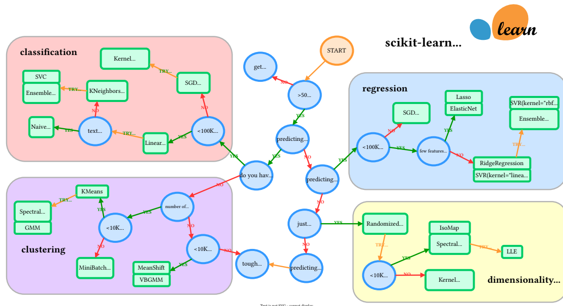
Figure 1: A cheatsheet of algorithms available in Scikit-Learn
