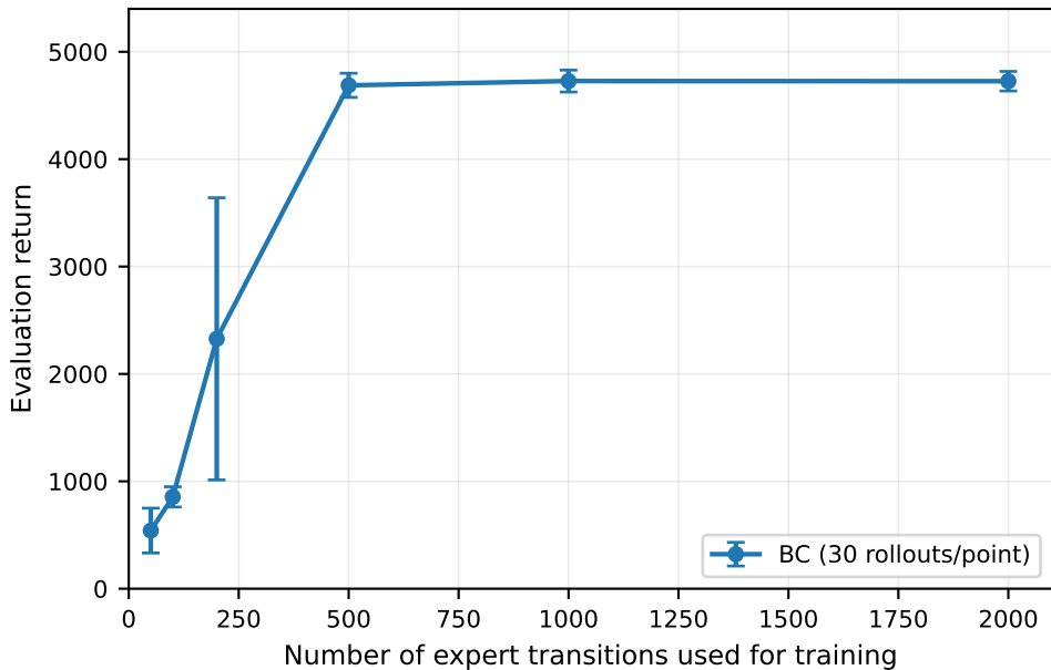
BC on Ant-v2 vs. amount of expert data
