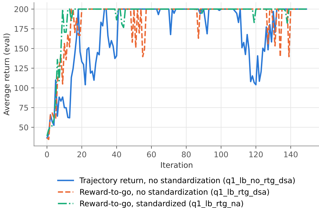
CartPole-v0, large batch ( b = 6000 )
