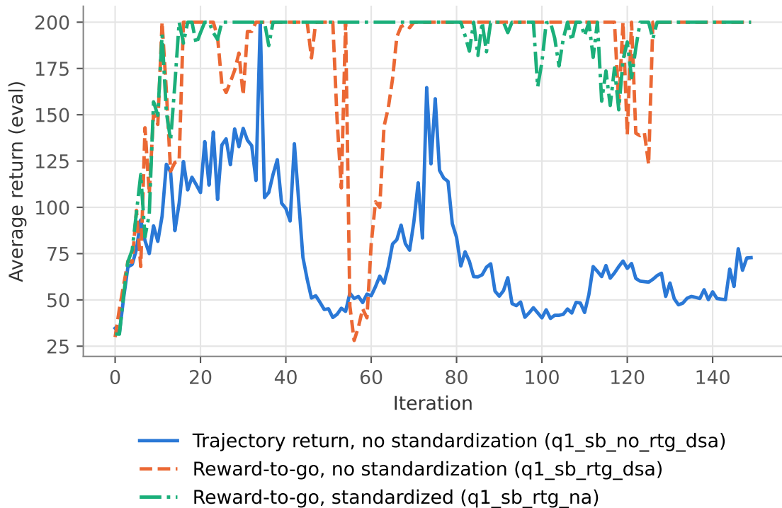
CartPole-v0, small batch (b = 1500)
