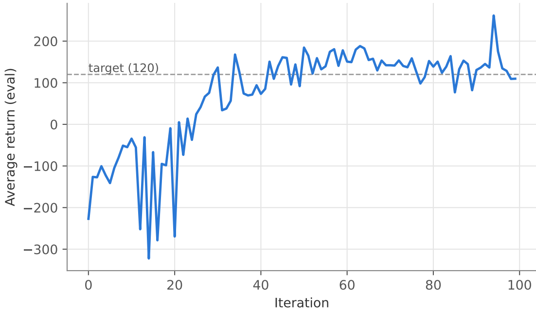
LunarLanderContinuous-v2, rtg + NN baseline (q3_b10000_r0.005)
