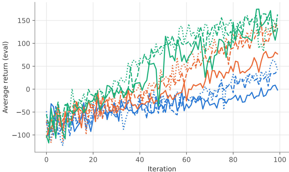
HalfCheetah-v4 search, rtg + NN baseline (q4_search_b<b>_lr<r>_rtg_nnbaseline)
