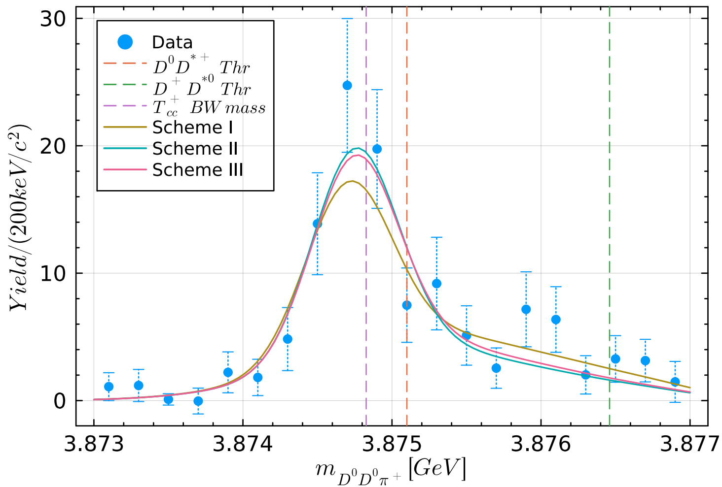
Distribution of D^0 D^0 \pi^+ with mass resolution
