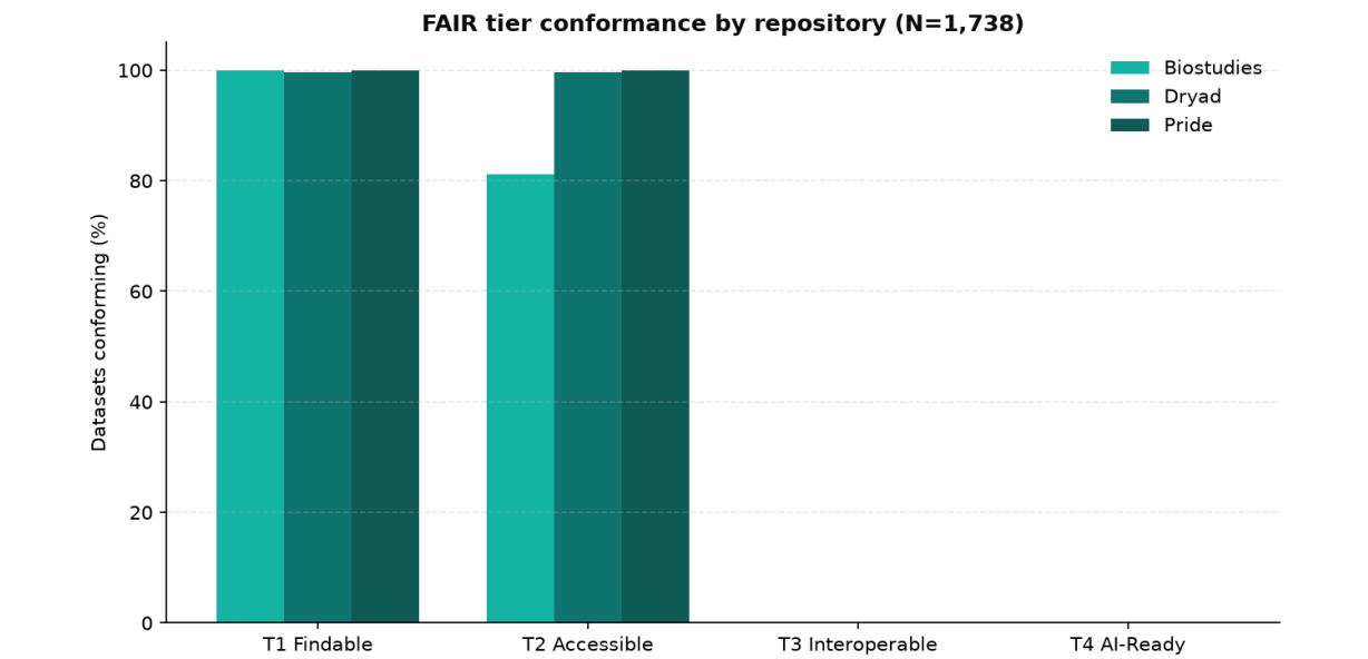
Tier conformance by repository
