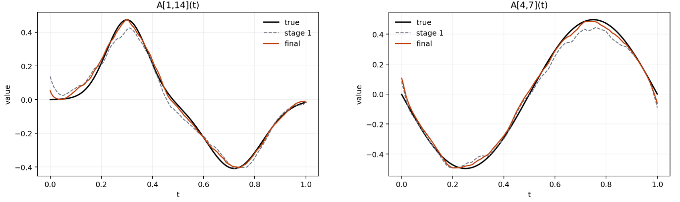
Figure 3: Selected estimated coefficient-function curves from Case 2.
