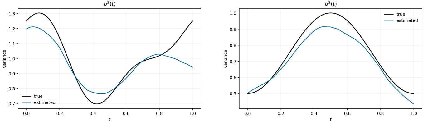
(a) True \sigma^2(t) = 1 + 0.25 \cos(2\pi t) + 0.1 \sin(4\pi t) .
