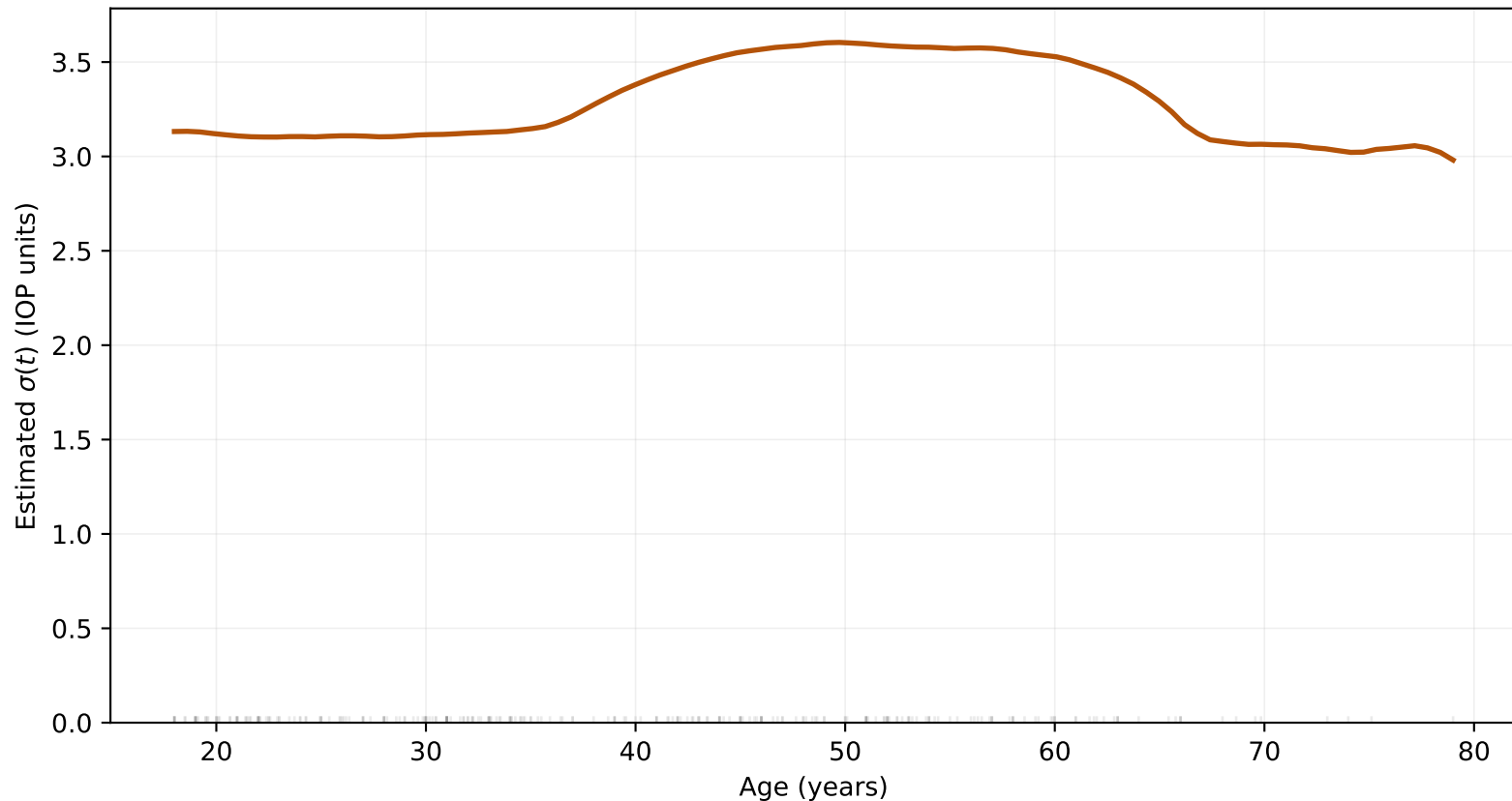
CFP full-sample sigma curve; h=1.8, hbar=0.25
