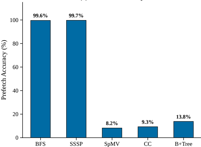
(a) Prefetch Accuracy
