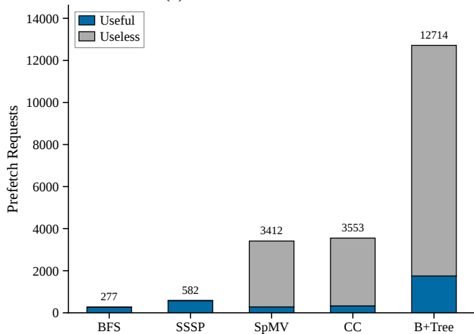
(b) Issued vs. Useful Prefetches
