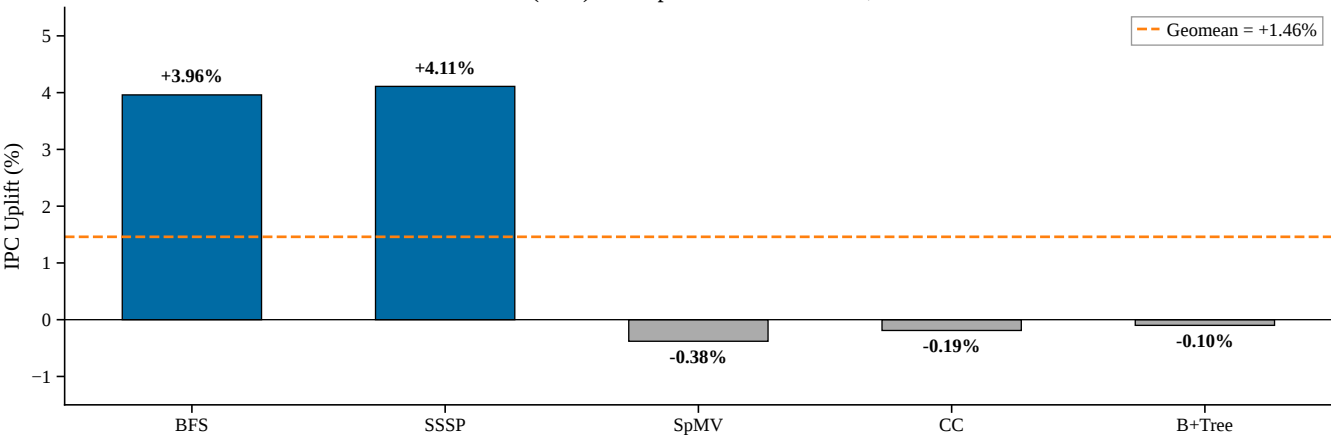
Stride Baseline (intra) IPC Uplift — 500k Window, All Workloads
