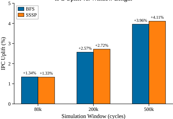
IPC Uplift vs. Window Length
