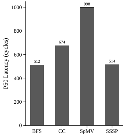
(c) Data Load Refill Latency
