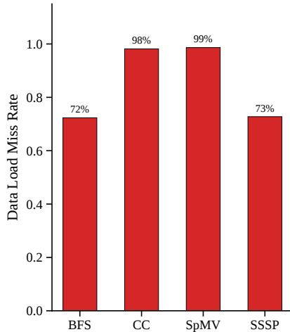
(b) Data Load L1 Miss Rate
