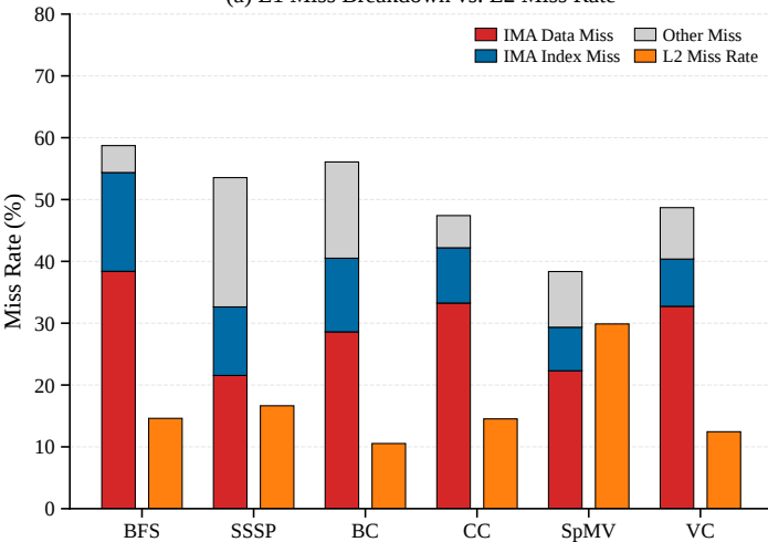
(a) L1 Miss Breakdown vs. L2 Miss Rate
