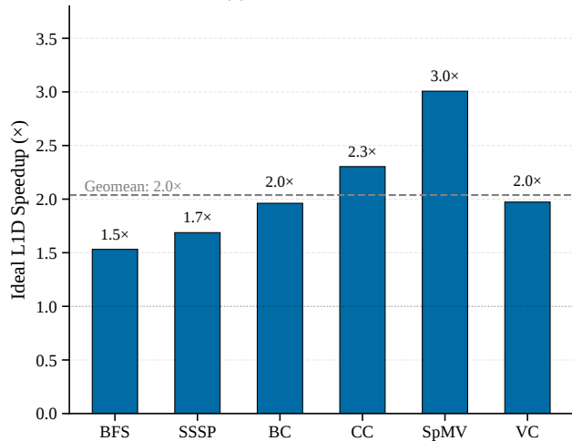
(b) Ideal L1D Headroom
