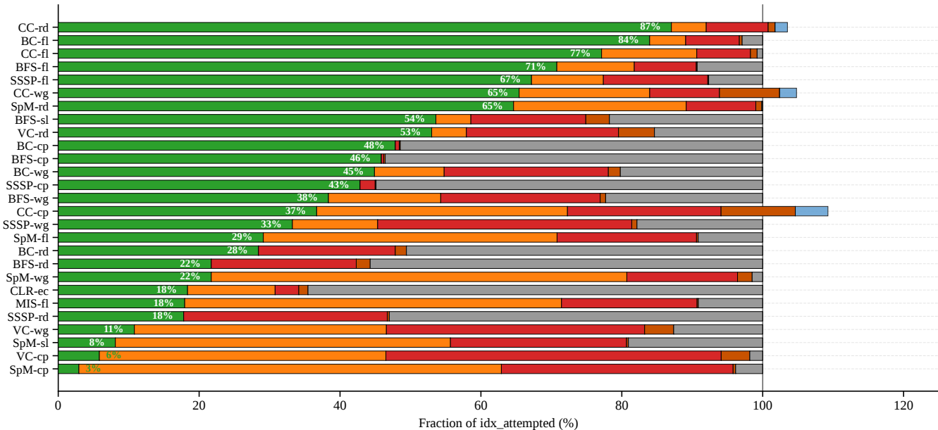
GRASP Pipeline Funnel: Idx Attempted -&gt; Delivered (mean delivery = 41%)
