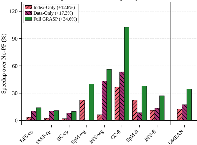
Component Ablation: IPC Speedup vs Baseline
