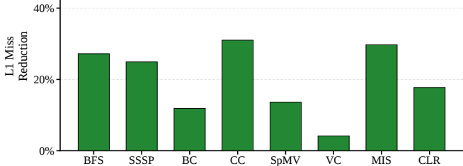
(a) L1 Miss Reduction
