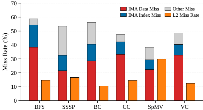
(a) L1 Miss Breakdown vs. L2 Miss Rate
