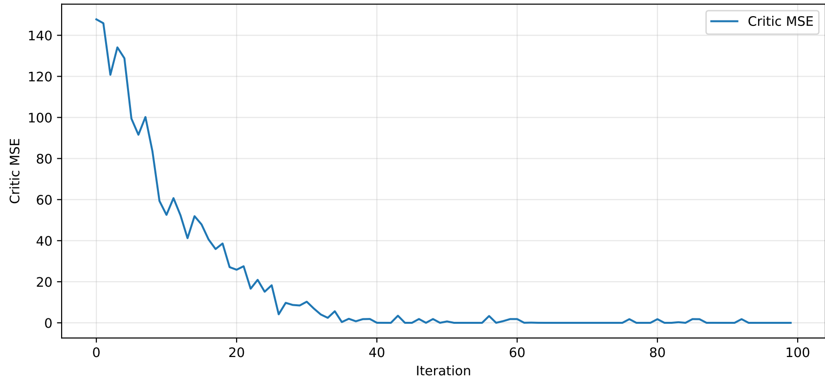
Value-baseline fit
