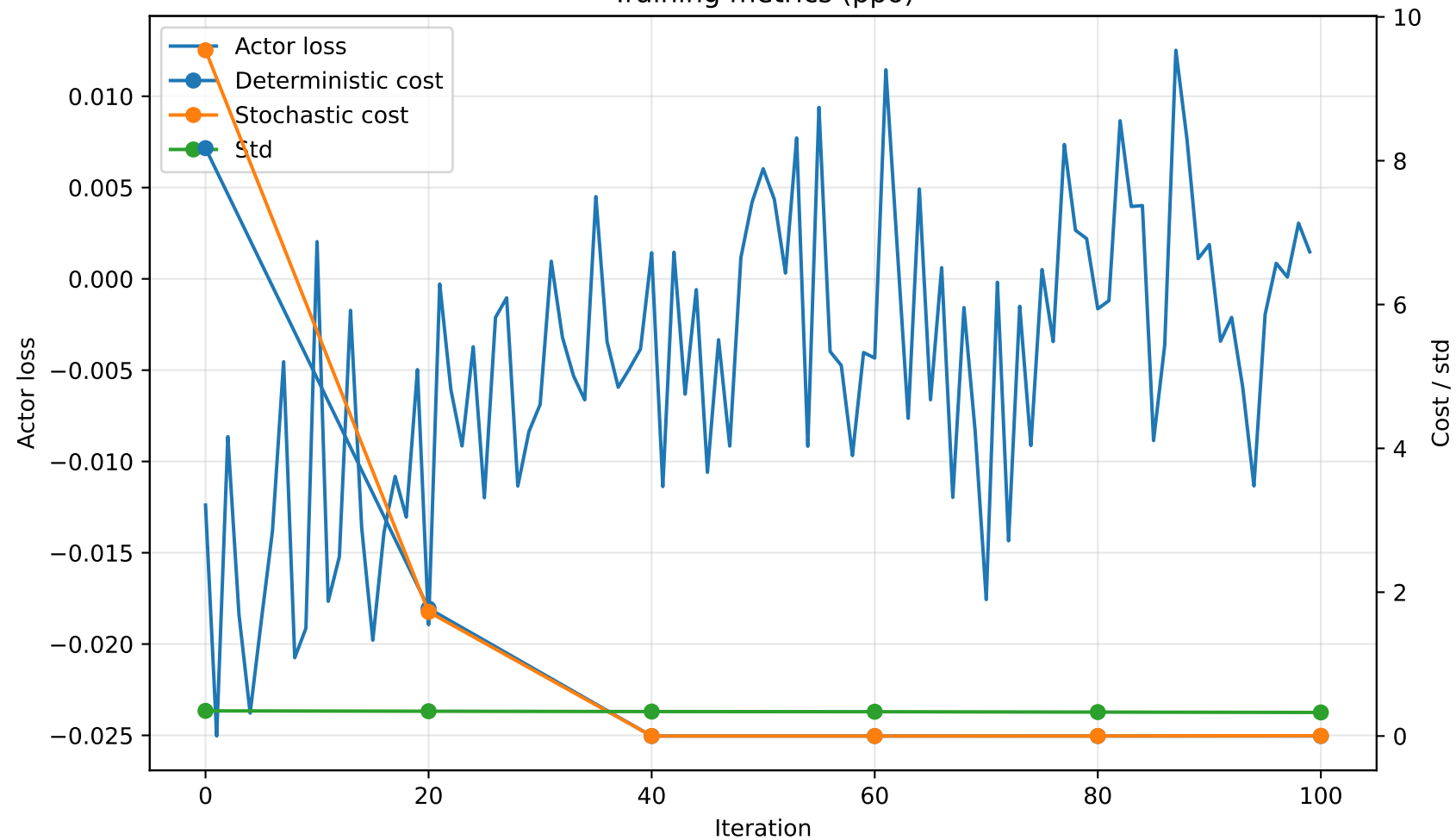
Training metrics (ppo)
