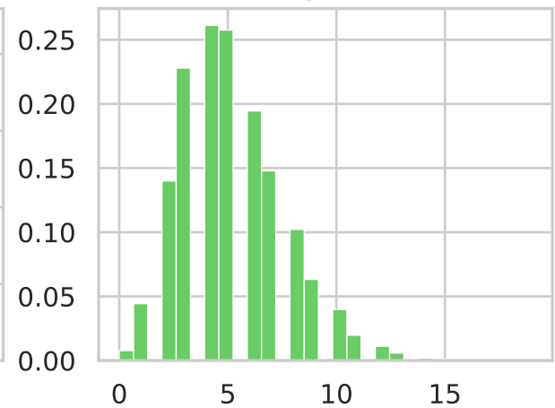
GraphVAE
