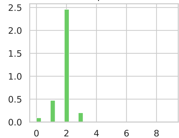
GraphVAE
