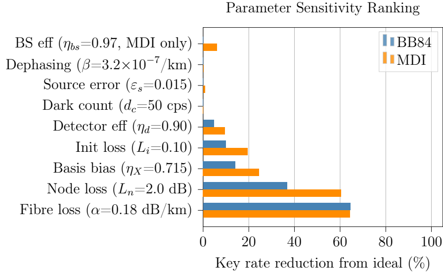
Figure 9: Percentage key-rate reduction from the ideal (layer-0) baseline at 25 km separation, for each parameter set individually to its layer-9 realistic value (Table 2). BS efficiency applies to MDI only; the BB84 bar is fixed at zero.
