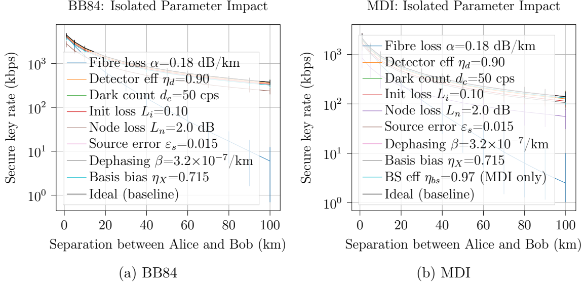
Figure 10: Secure key rate versus Alice–Bob separation with exactly one hardware parameter set to its layer-9 realistic value (Table 2) and all others held ideal, against an ideal (baseline) reference. Error bars show the Monte Carlo sample spread.
