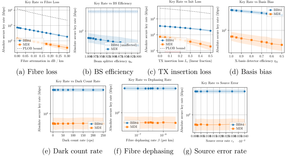
Figure 11: Remaining point-to-point parameter sweeps. BB84 in blue (circles), MDI in orange (squares); shaded bands show Monte Carlo sample spread. Except for the parameter swept in each panel, all hardware parameters take their layer-9 default values from Table 2.
