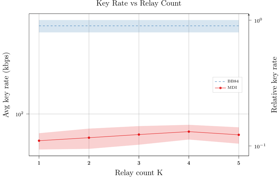
Figure 11: Mean key rate versus relay count K for N = 15 users in a 25 \times 25 km service area, averaged over 5 independent seeds; shaded bands show the spread across seeds. BB84 is relay-independent (dashed baseline, 614.3 kbps). The right axis shows MDI’s rate relative to the BB84 baseline at each K .
