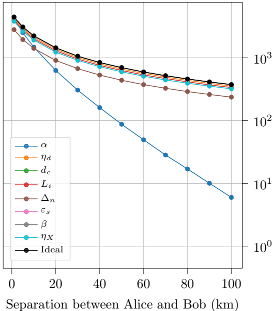
(a) BB84
