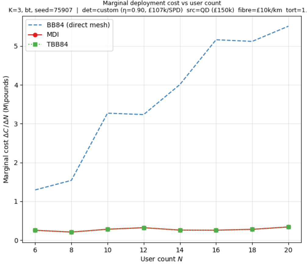
Figure 18: Marginal deployment cost, \Delta C/\Delta N , for the BT London topology. BB84’s marginal cost rises with N ; MDI’s and TBB84’s stay flat and low throughout.
