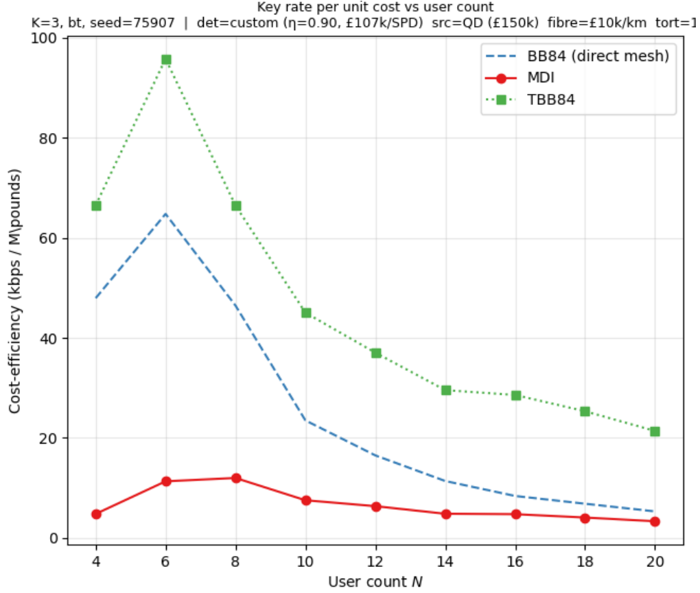
Figure 17: Key rate per unit deployment cost (kbps/£M) for the BT London topology. TBB84 and BB84 both substantially outperform MDI on this metric, since MDI’s lower absolute cost (Figure 16) is more than offset by its much lower key rate (Section 5.1).
