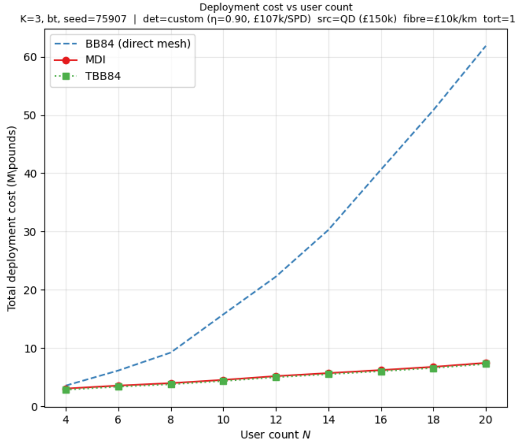
Figure 16: Total deployment cost against user count N for the BT London topology ( K = 3 ). BB84’s direct mesh diverges quadratically; MDI and TBB84 stay low and nearly coincide, consistent with the N^* ceiling of at most K + 1 = 4 users derived analytically in Section 4.3 for this K .
