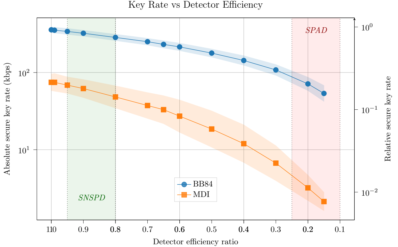
Figure 5: Absolute and relative secure key rate versus detector efficiency \eta_d , at fixed 20 km separation and 0.18 dB/km attenuation. Shaded bands mark typical SNSPD (IDQ ID281) and InGaAs SPAD (IDQ ID230) operating ranges.
