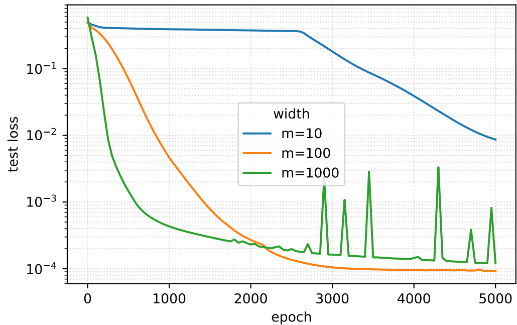
Training curves — target=sin_low, seed=0
