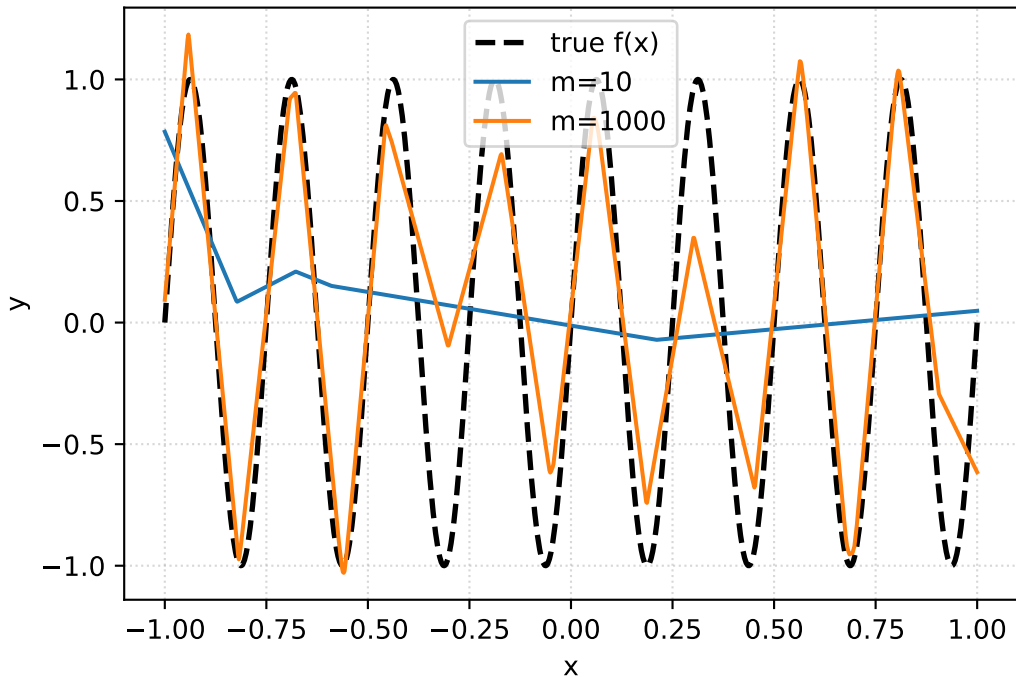
Learned vs true — target=sin_high, seed=0
