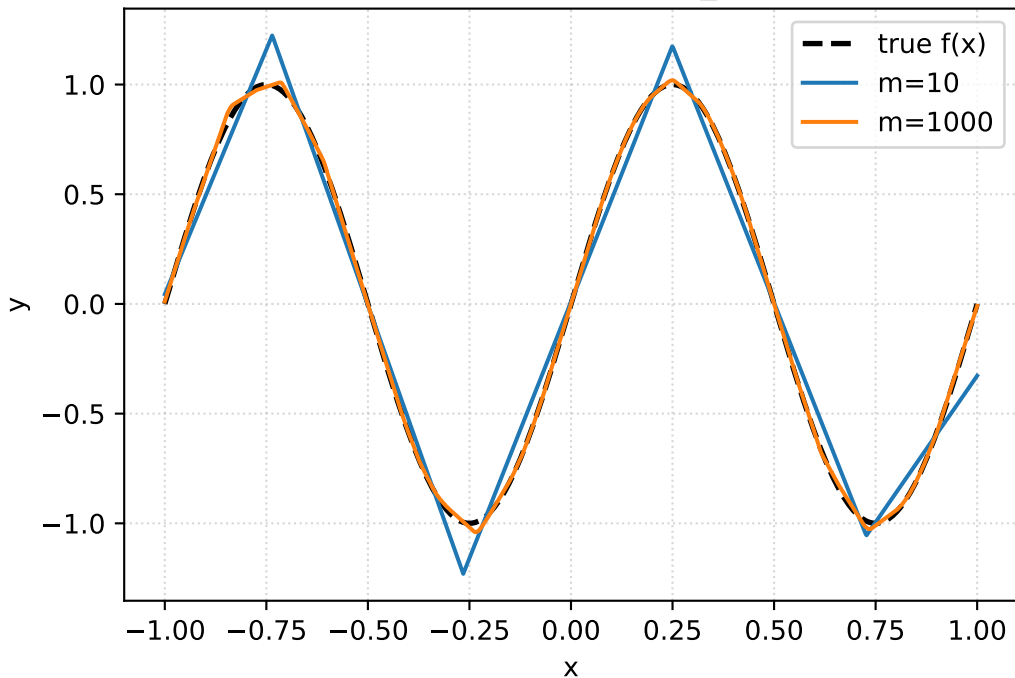
Learned vs true — target=sin_low, seed=0
