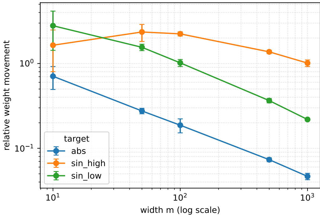
Lazy training: relative movement vs width
