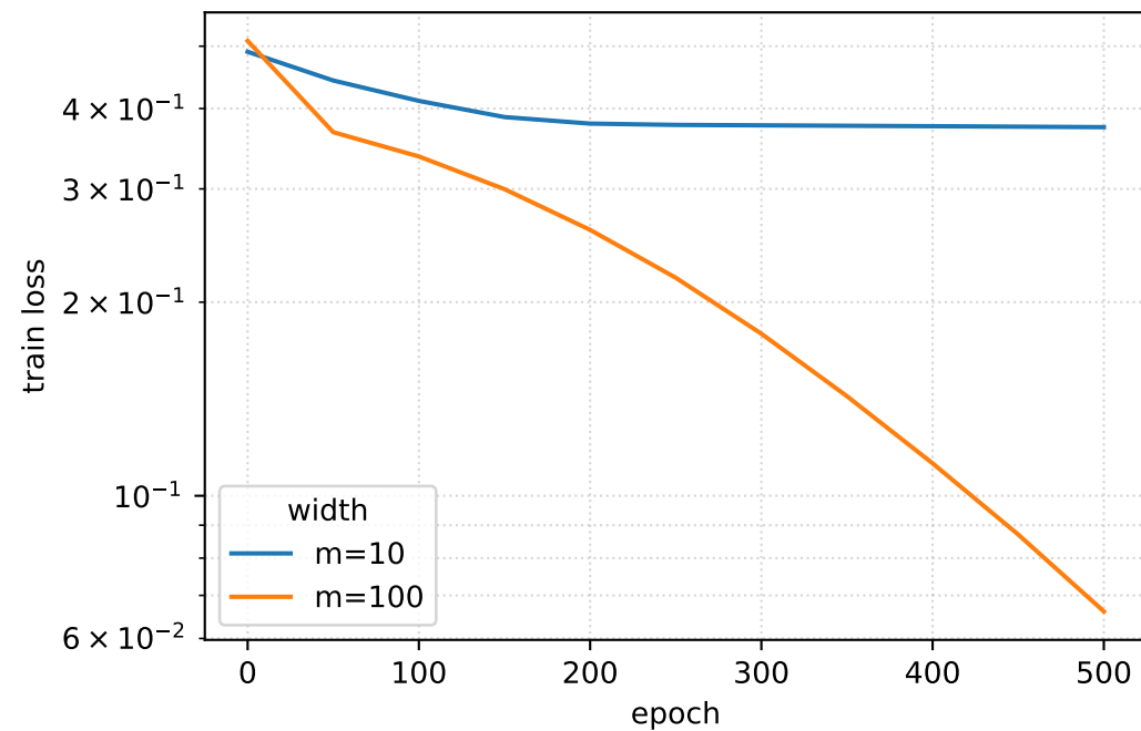
Training curves — target=sin_low, seed=0
