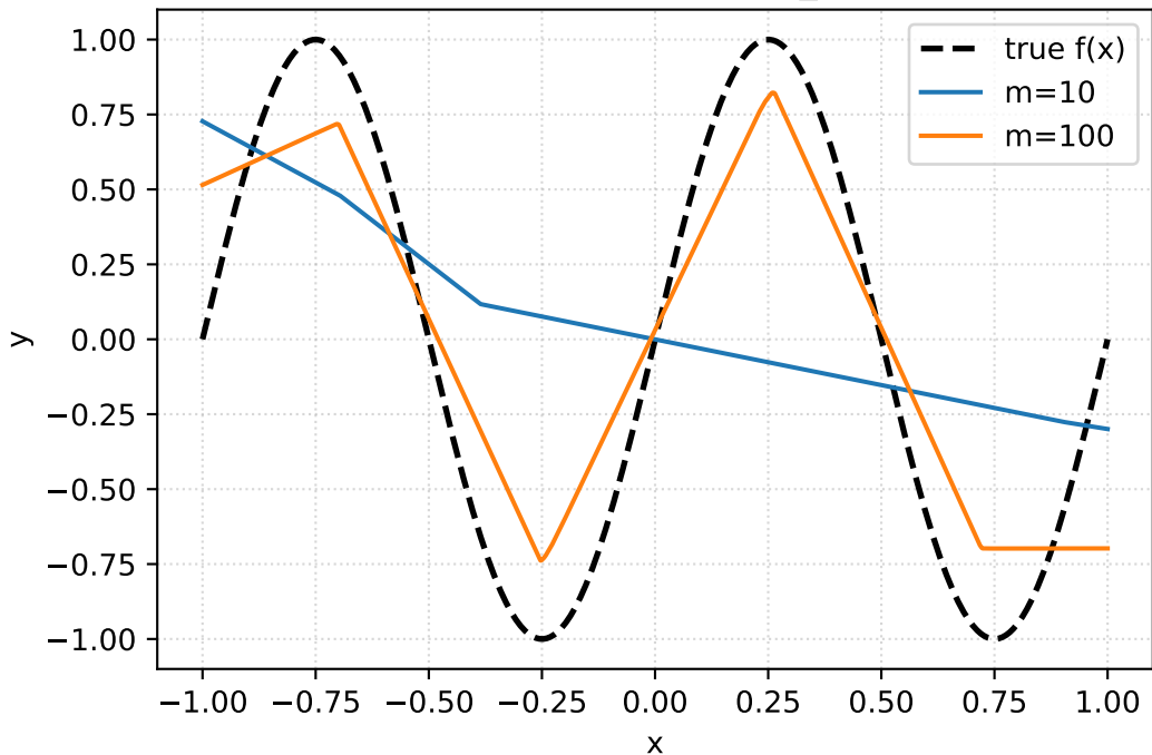
Learned vs true — target=sin_low, seed=0
