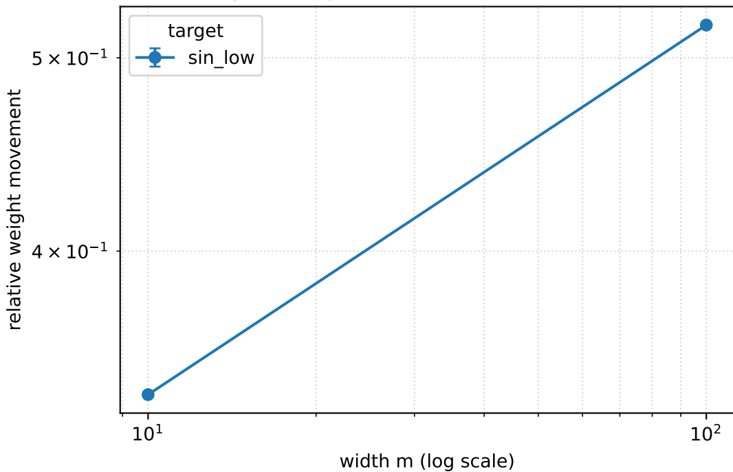
Lazy training: relative movement vs width
