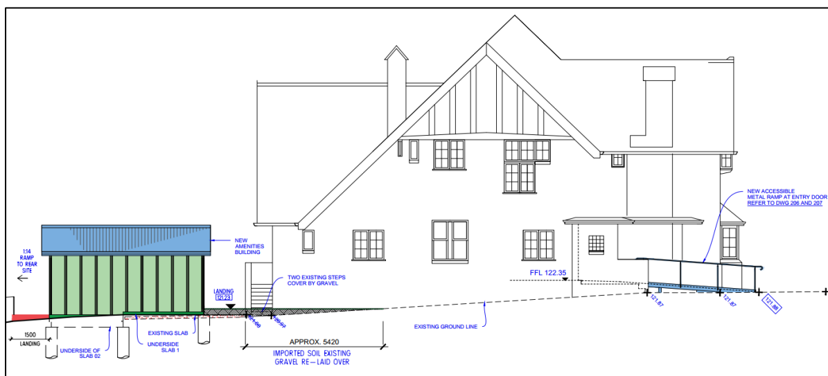
Figure 3: Extract of Northern Elevation, proposed works shown in colour (Source Lucas Stapleton Johnson, 08.01.2025)
