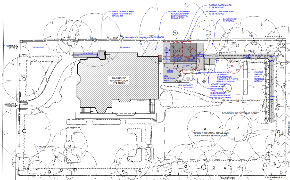
Figure 2: Extract of proposed Site Plan, new works shown in grey (Source Lucas Stapleton Johnson, 08.01.2025)
