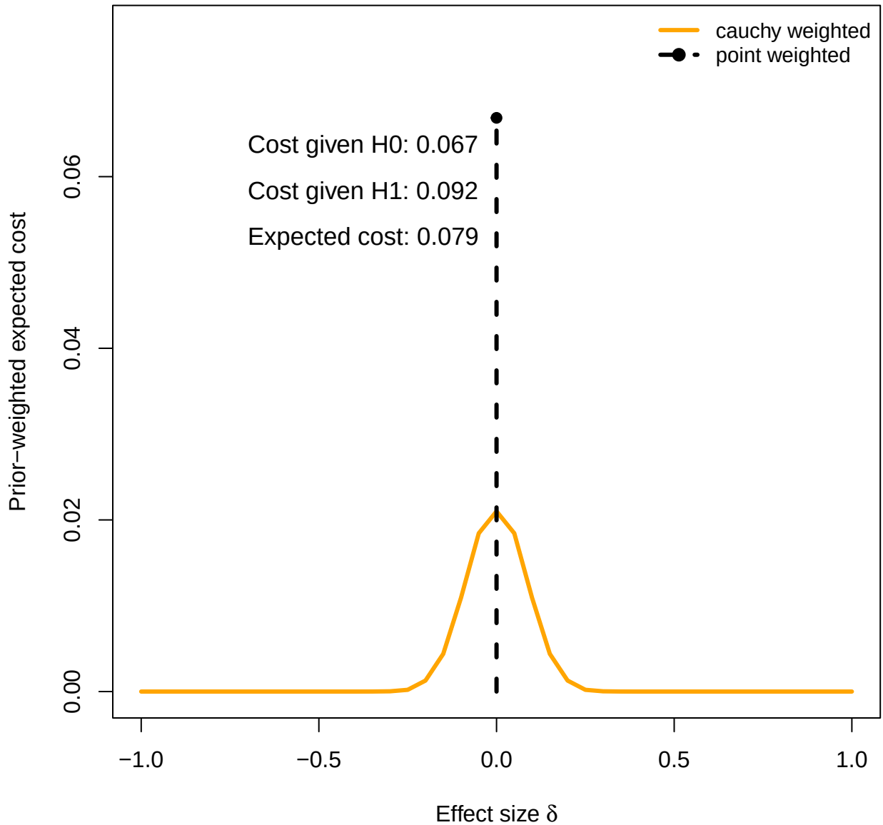
Prior-weighted expected cost (Optional Stopping), r=0.707 , BF_{crit}=10
