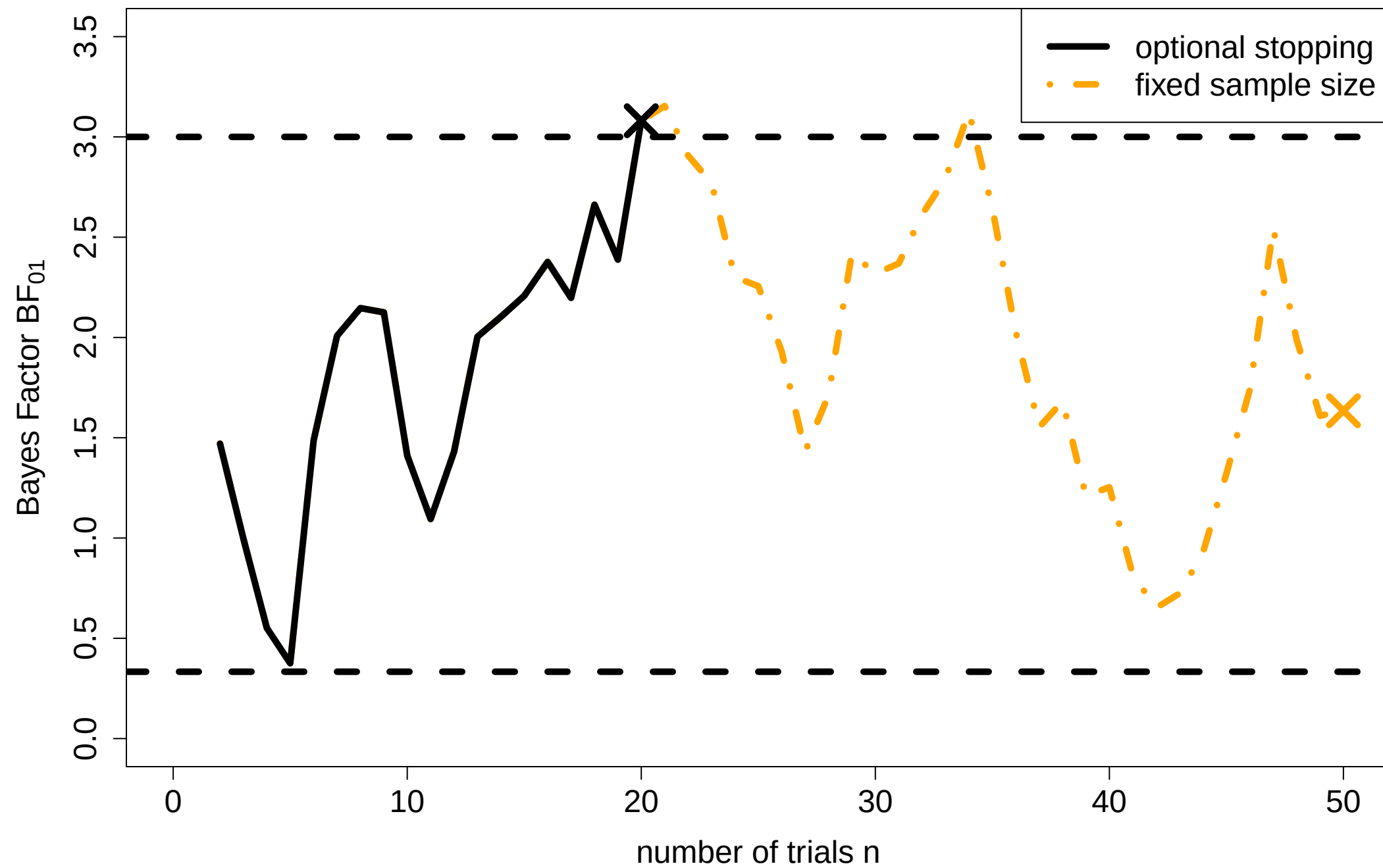
Fixed Sample Size vs Optional Stopping
