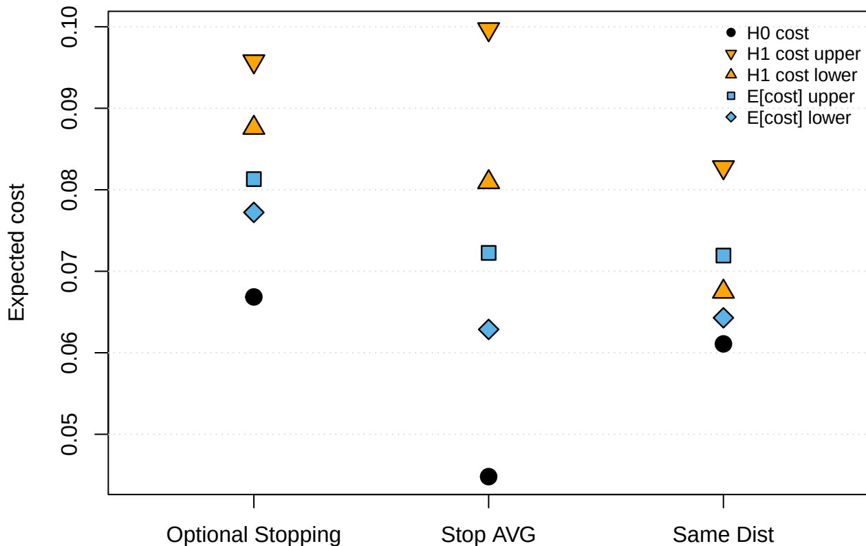
Expected costs overview (BF_crit = 10)
