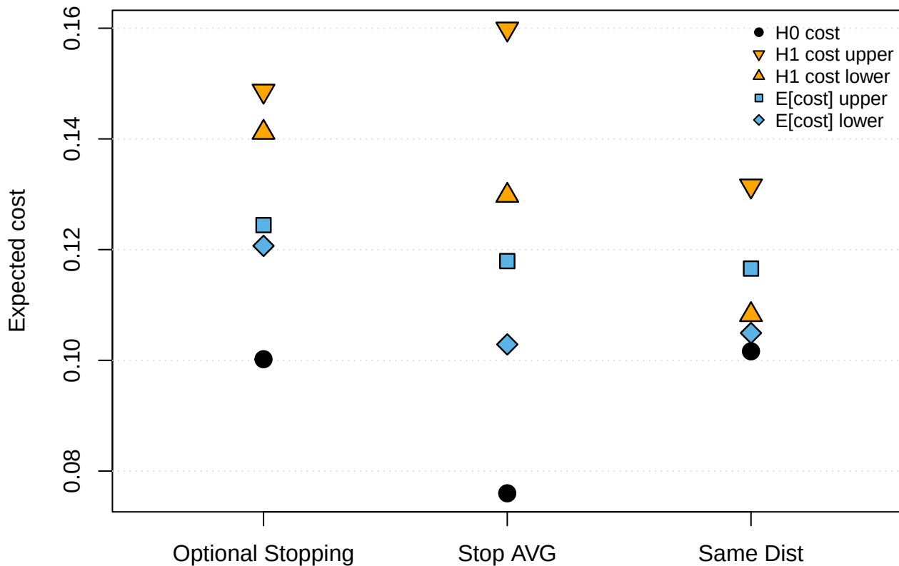
Expected costs overview (BF_crit = 6)
