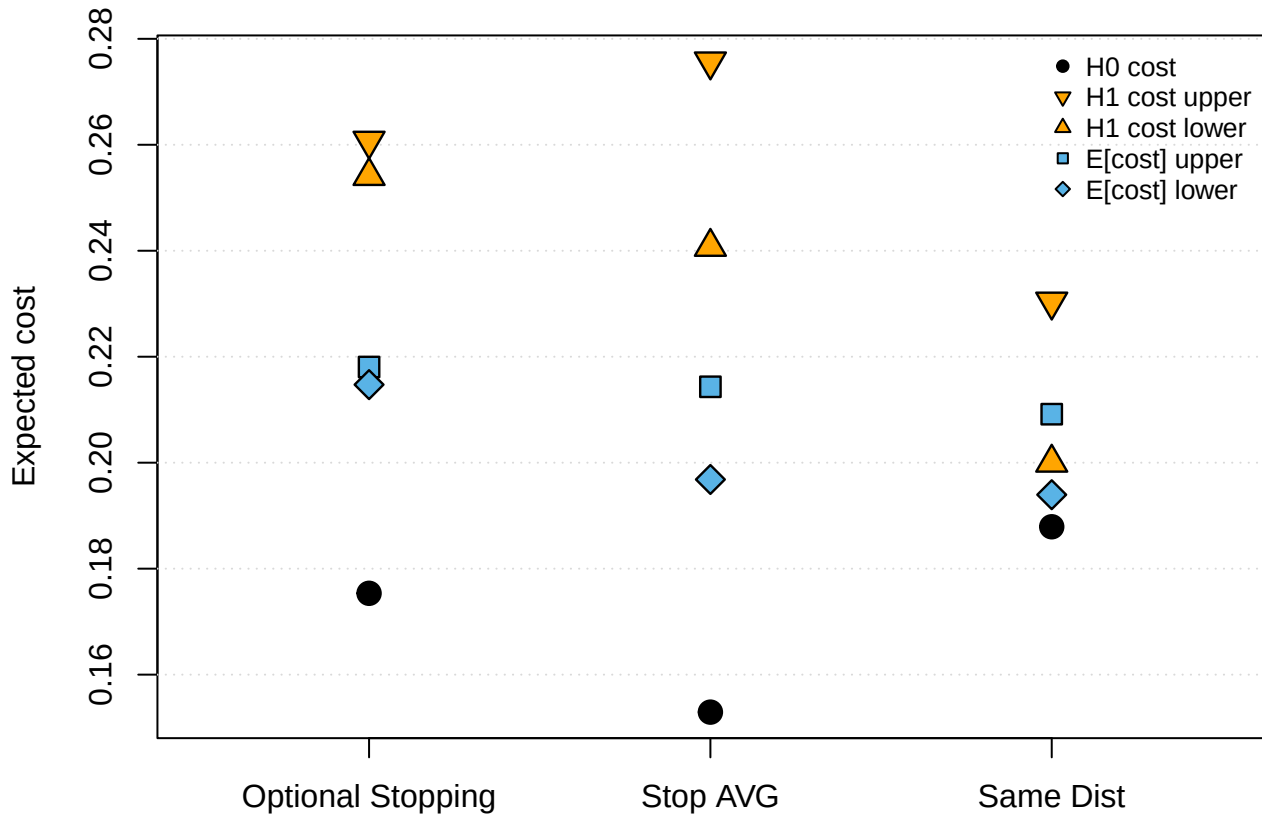
Expected costs overview (BF_crit = 3)
