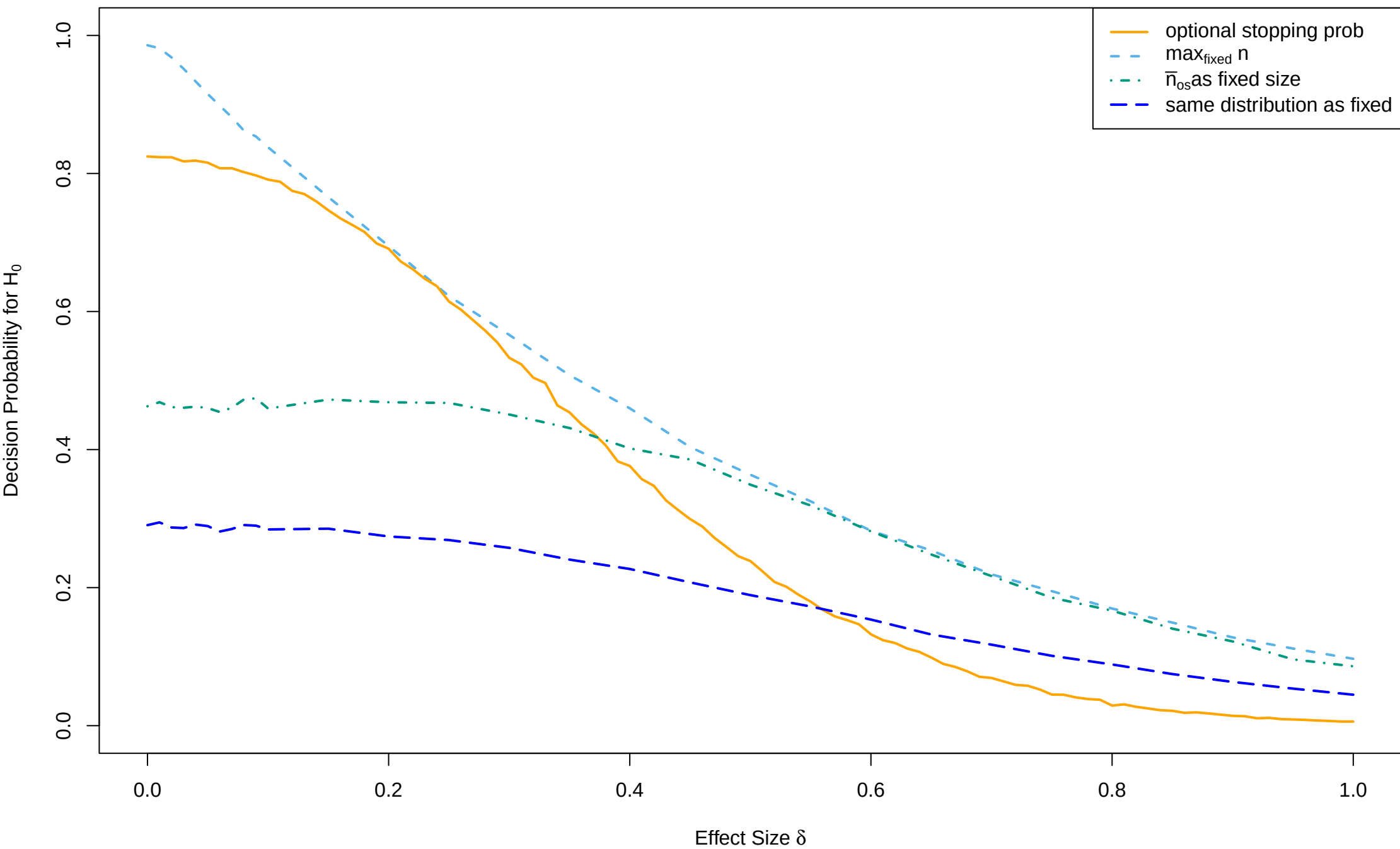
Fixed Size vs Optional Stopping for BF_{\text{crit}} = 3 , r = 0.7071068
