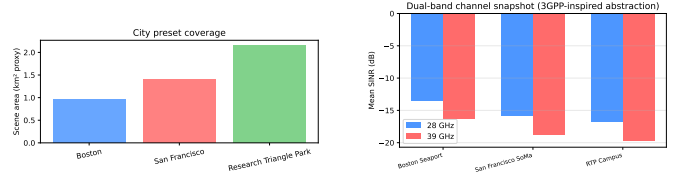
Fig. 2. Left: open-license city preset extents. Right: mean dual-band SINR (28/39 GHz) across presets.
