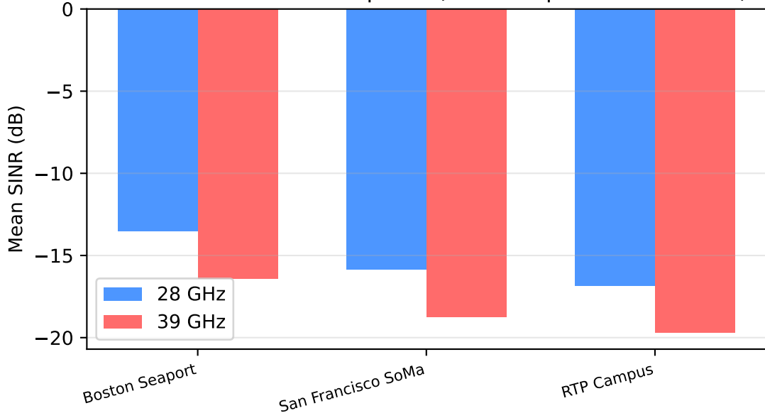
Dual-band channel snapshot (3GPP-inspired abstraction)
