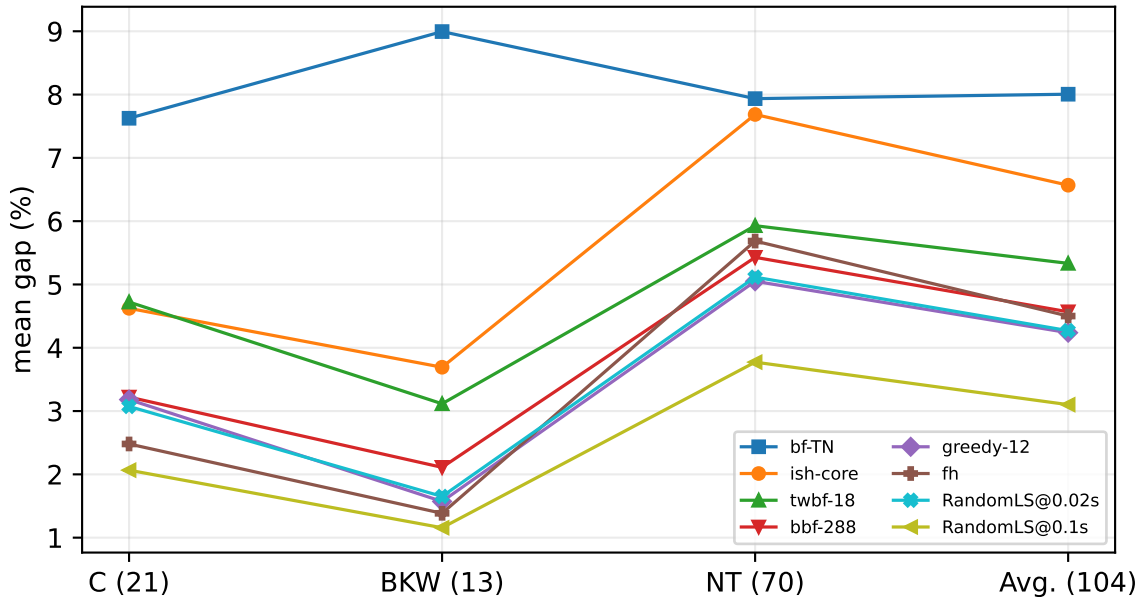
Mean gap by instance family (RandomLS = five-seed mean)
