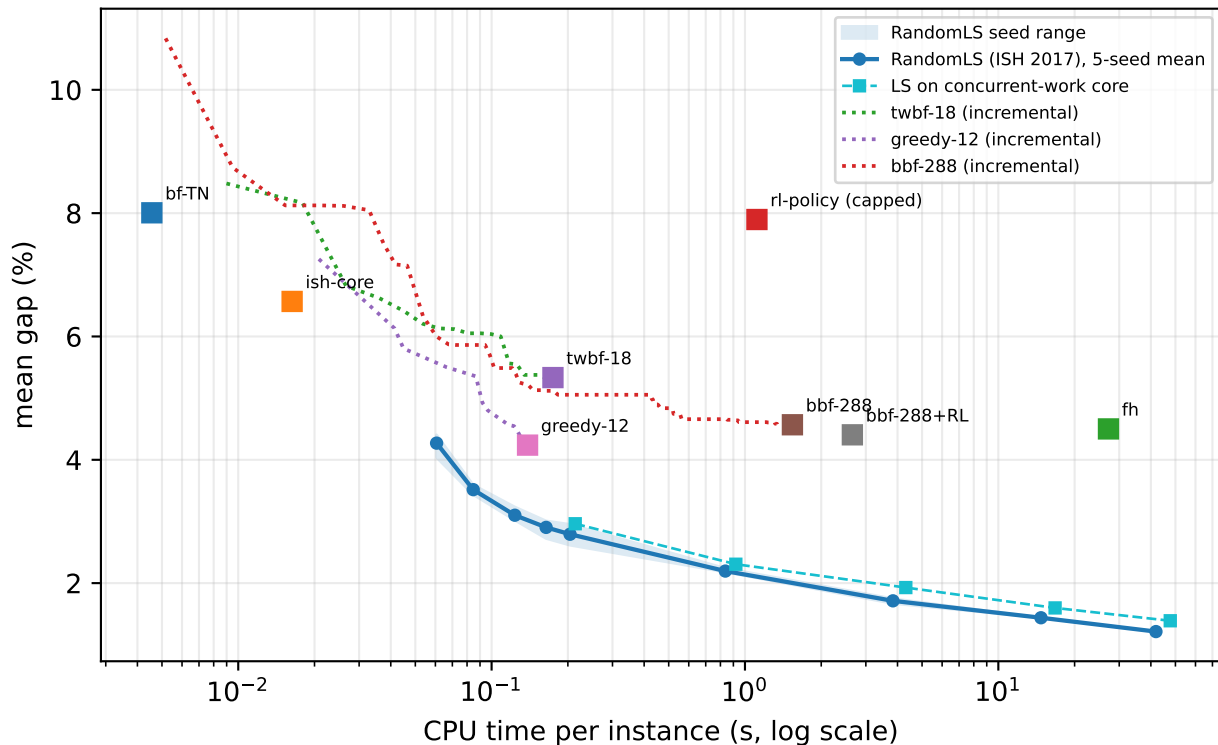
Cost--quality plane, 104 instances (instance-count weighted)
