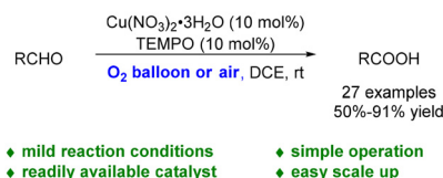
Scheme 1 Copper catalyzed oxidation of aldehydes to acids.
