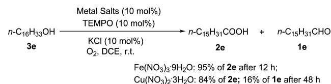
Scheme 1. Aerobic Oxidation of 3e with Different Metal Nitrates
