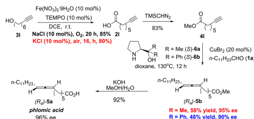
Scheme 5. Total Synthesis of Phlomic Acid Using Aerobic Oxidation and EATA
